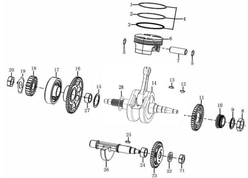
曲轴连杆部件/活塞 CRANKSHAFT CONNECTING-ROD
