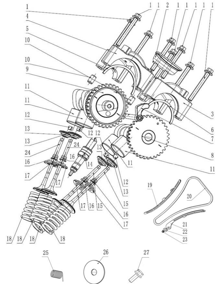
配气机构 VALVE MECHANISM
