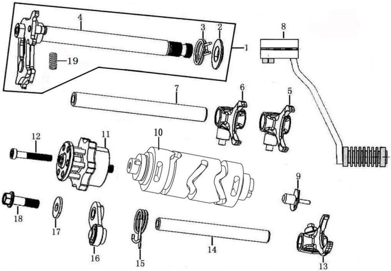
变速机构 GEARSHIFT MECHANISM
