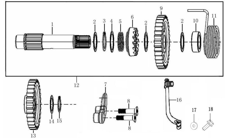
启动轴总成 KICK STARTING SHAFT ASSEMBLY
