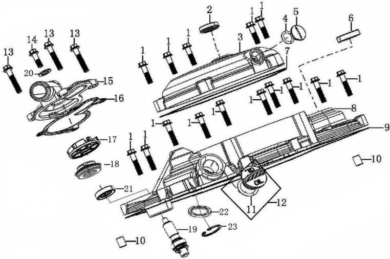
右曲轴箱盖 RIGHT CRANKCASE COVER
