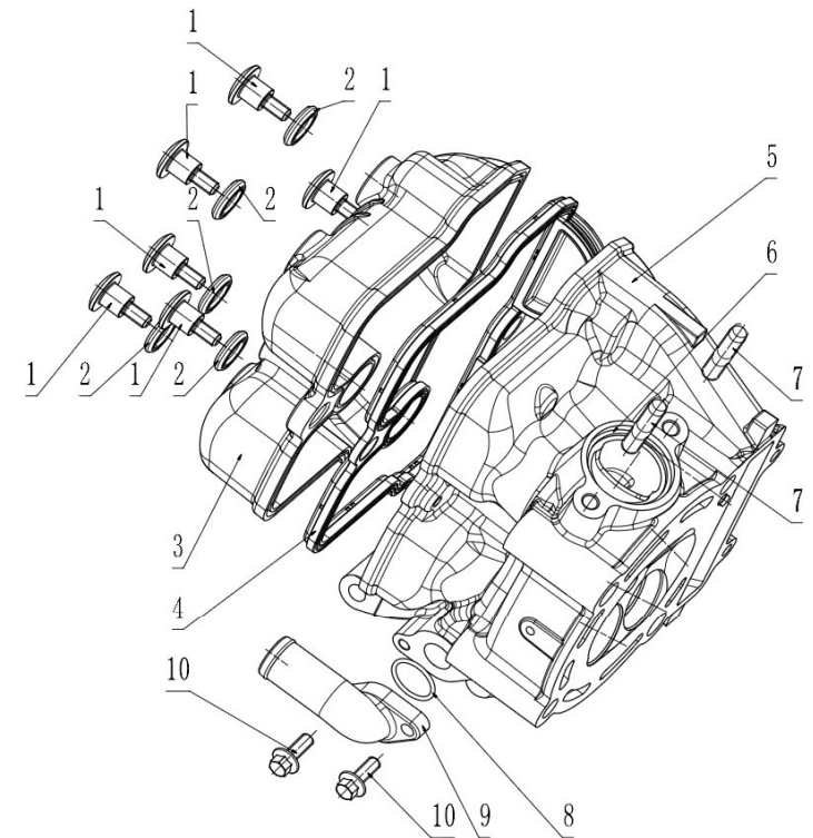
气缸头部件 CYLINDER HEAD ASSY
